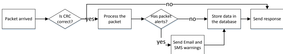
Figure 5. Flow chart of the server side pre-processor script
