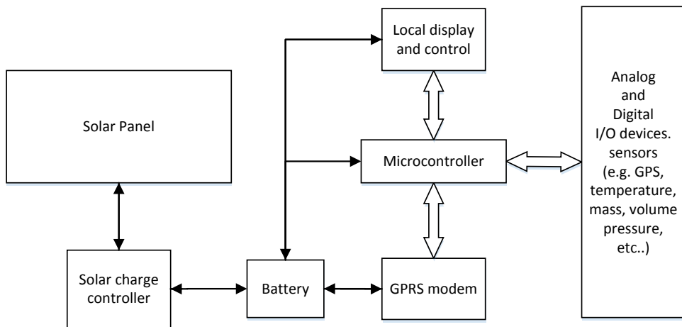
Figure 4. Components of the remote system
