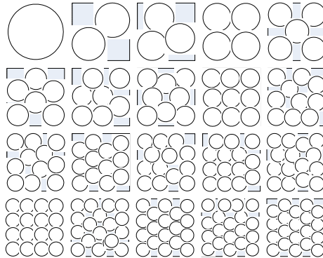
Figure 3. Location of circles in trivial square [3.]
