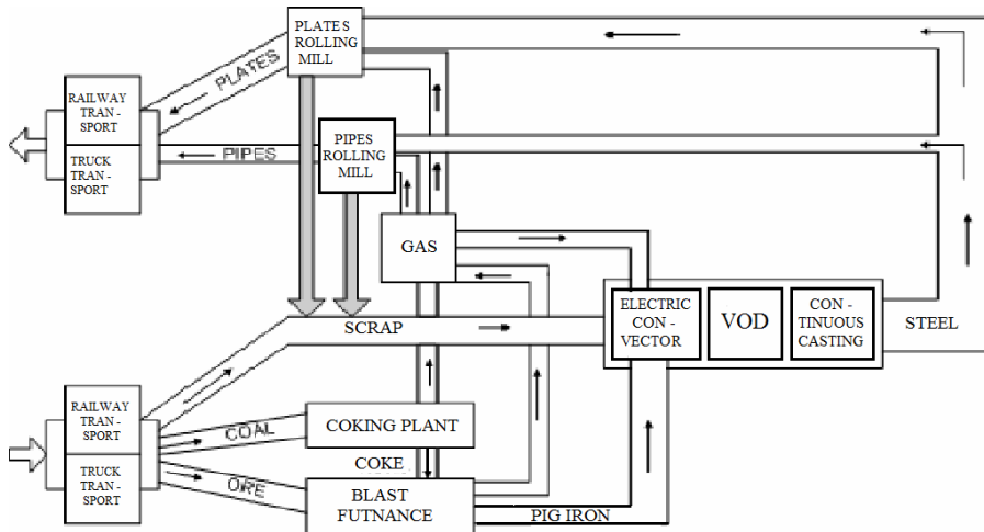
Figure 1. The system of the internal flow of material goods (materials and raw materials) in the metallurgical enterprise
