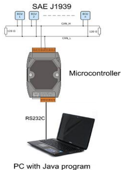
Figure 1. Measurement system
