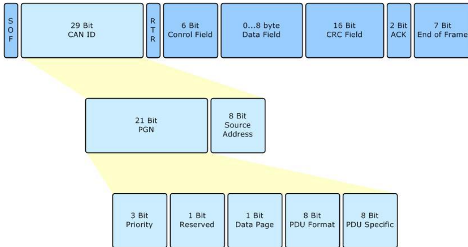
Figure 3. The structure of a CAN message
